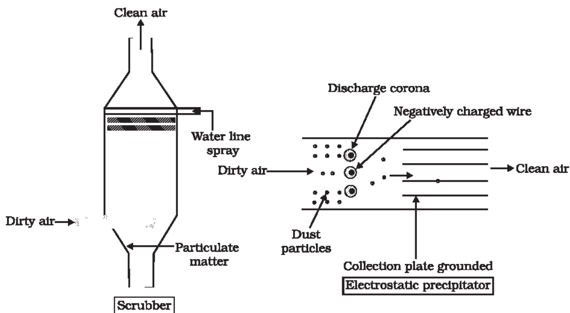
Figure 16.1 Electrostatic precipitator
